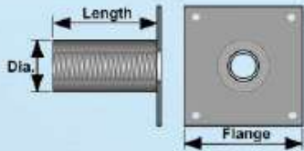
BPI® BARSPLICER FLANGED COUPLER
