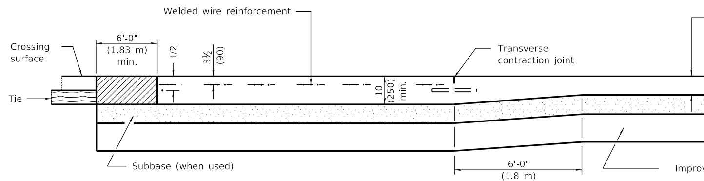
SECTION A-A (FOR PCC PAVEMENT)
