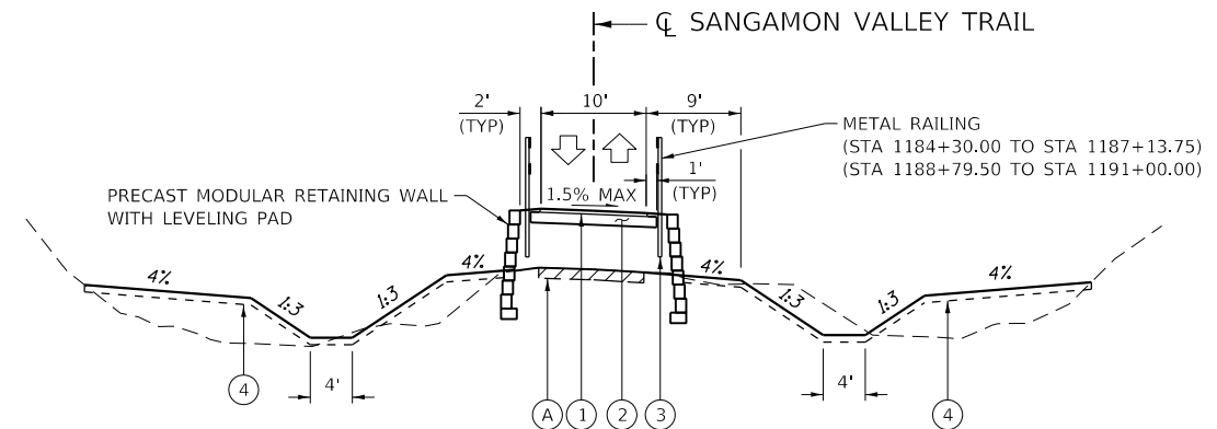
SANGAMON VALLEY TRAIL PROPOSED SECTION (STA 1184+65.0 TO STA 1187+13.7) (STA 1188+79.5 TO STA 1191+00.0) BRIDGE OMISSION STA 1187+13.7 TO 1188+75.5
