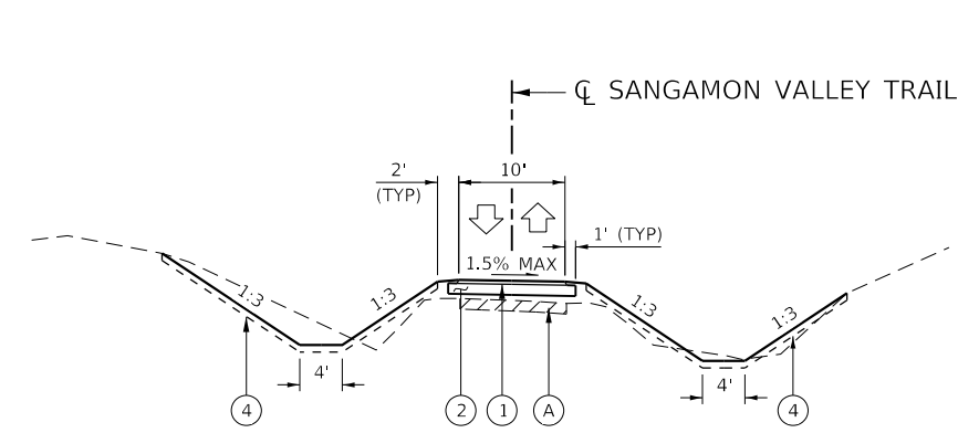
SANGAMON VALLEY TRAIL PROPOSED SECTION (STA 1183+00.0 TO STA 1184+65.0) (STA 1191+00.0 TO STA 1193+00.0)
