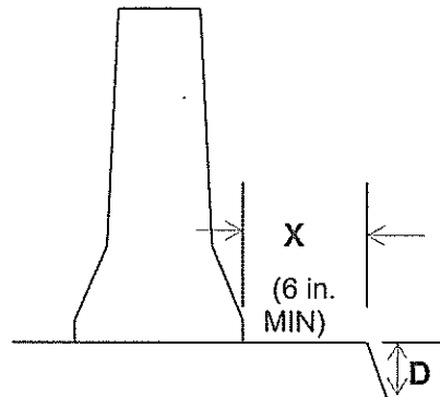
“Illinois F-Shape” TCB (Highway Standard 704001)
