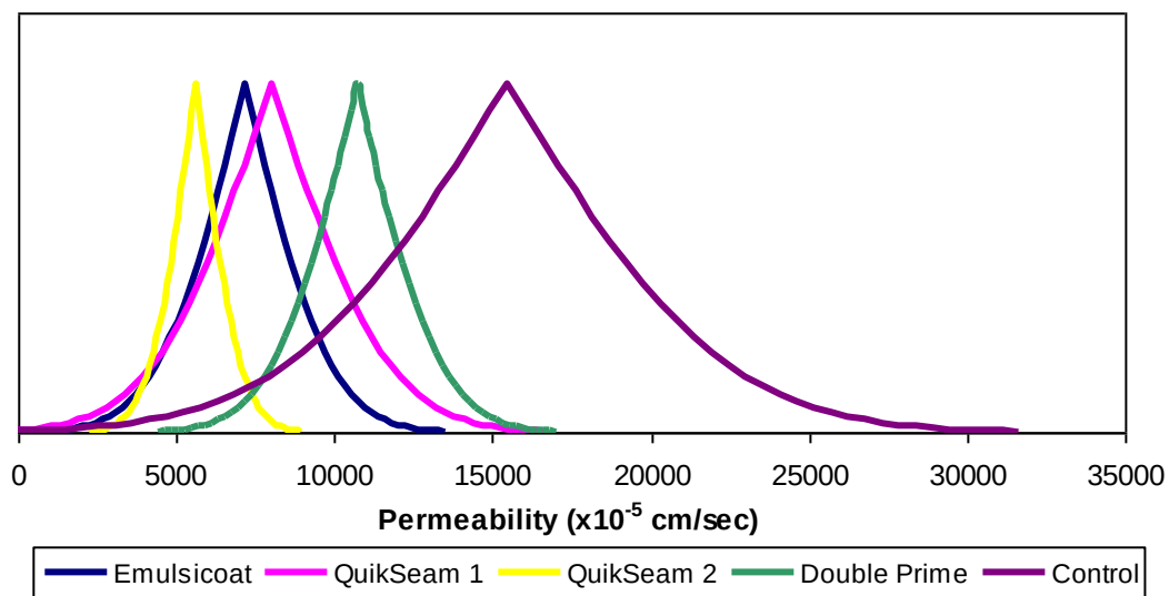
Figure 49: Joint Sealant Normal Distributions
