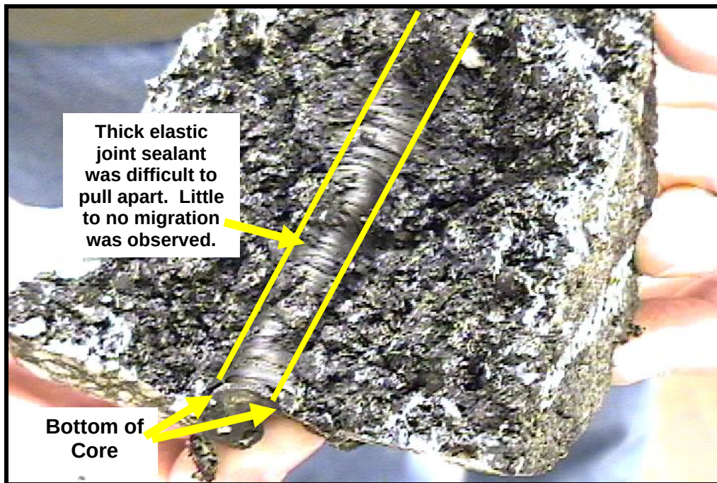
Figure 28: IL 40 Joint Sealant Migration (Thick Layer – No Migration)
