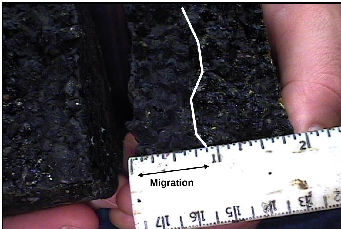
Figure 12: Joint Sealant Migration
