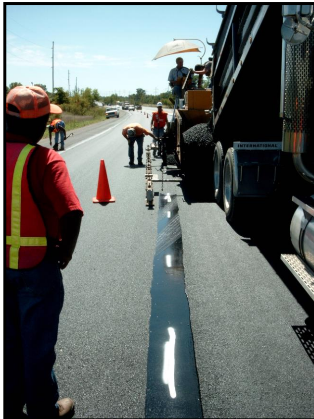
Figure 40: Paving over Jband
