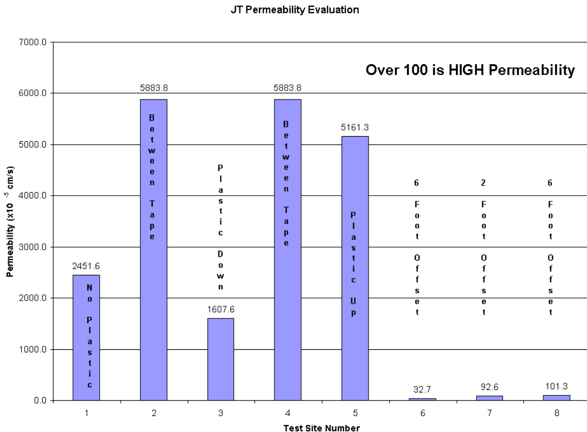
Figure 23: IL 10/121 Permeability Results
