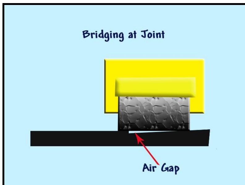
Figure 3: Roller Bridging at Joint
