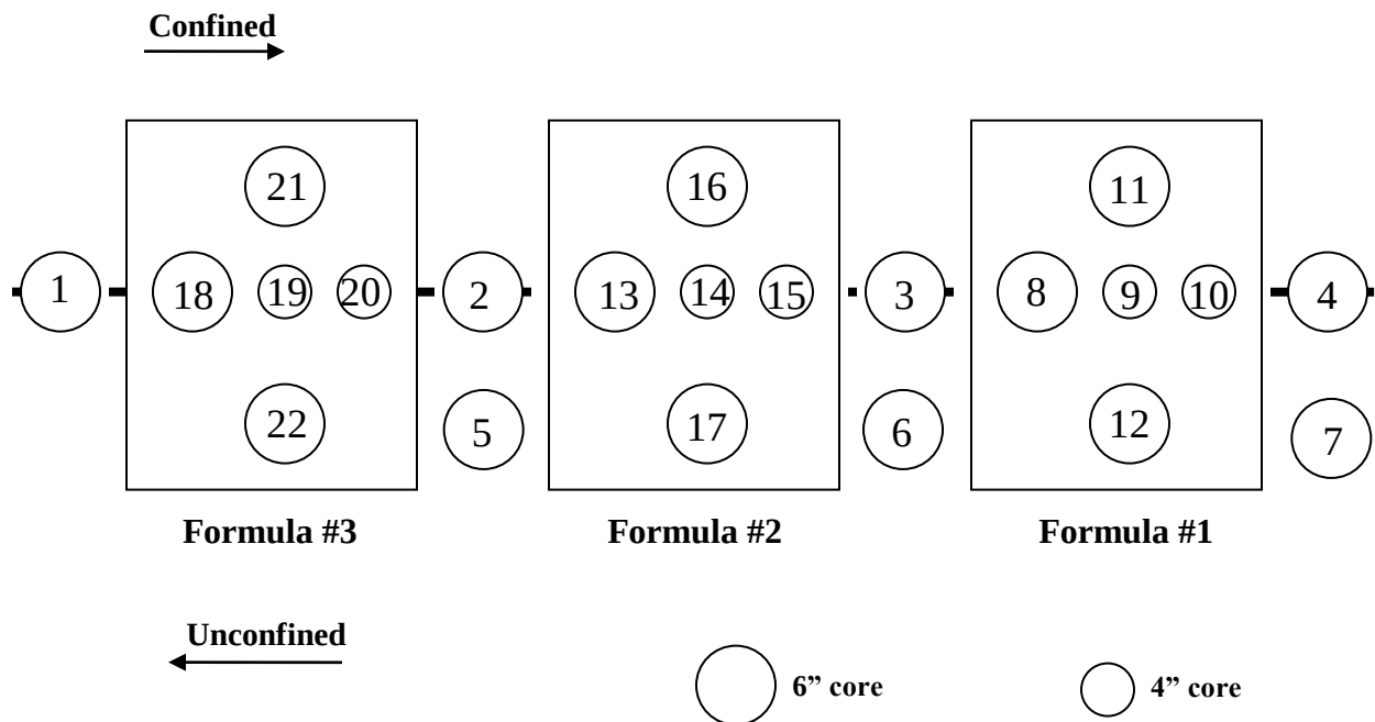
Figure 26: IL 40 Joint Testing Detail
