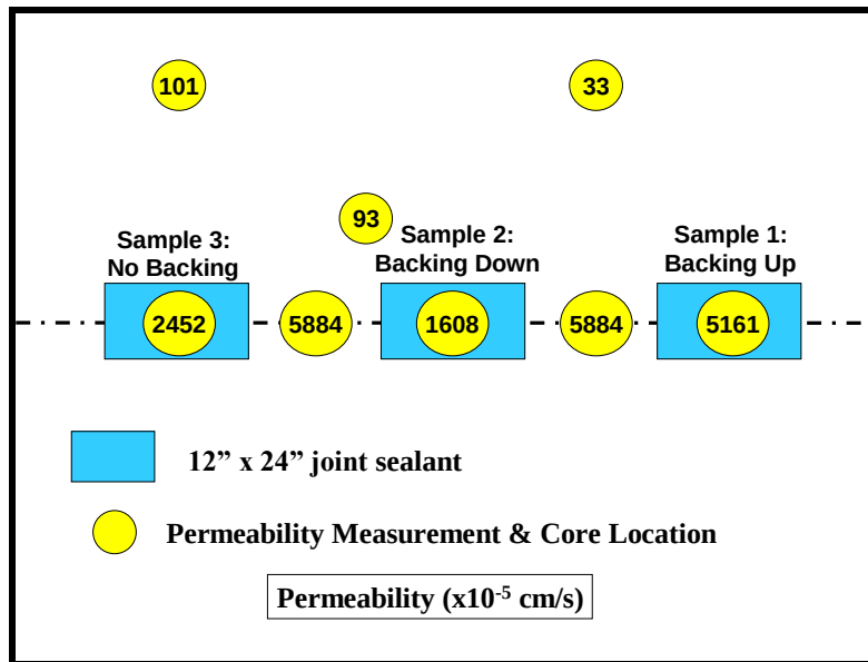
Figure 20: Testing Layout and Permeability Results
