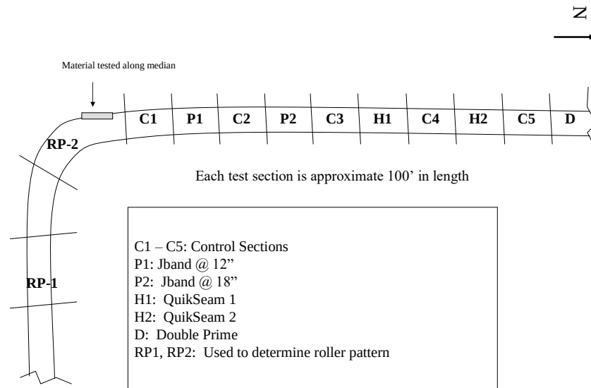
Figure 38: US 51 Test Section Layout
