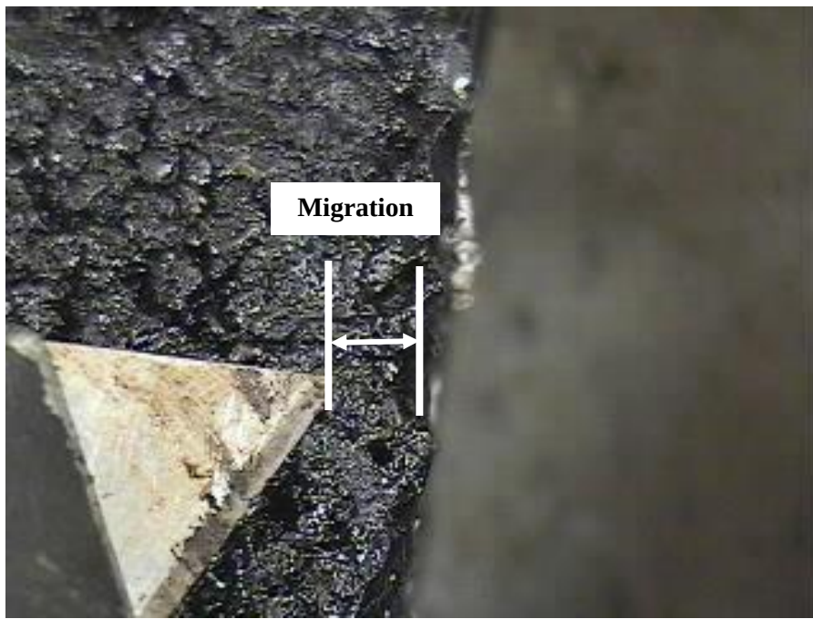
Figure 58: 4004 Side View
