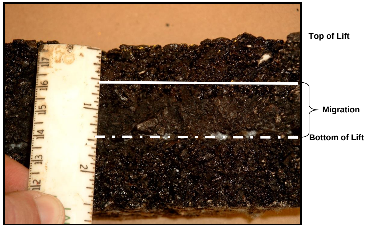
Figure 52: QuikSeam Formula 2 Migration
