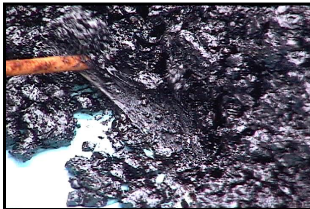
Figure 18: Joint Sealant Elasticity
