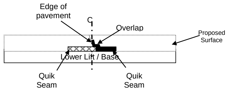
Figure 43: QuikSeam Typical Layout
