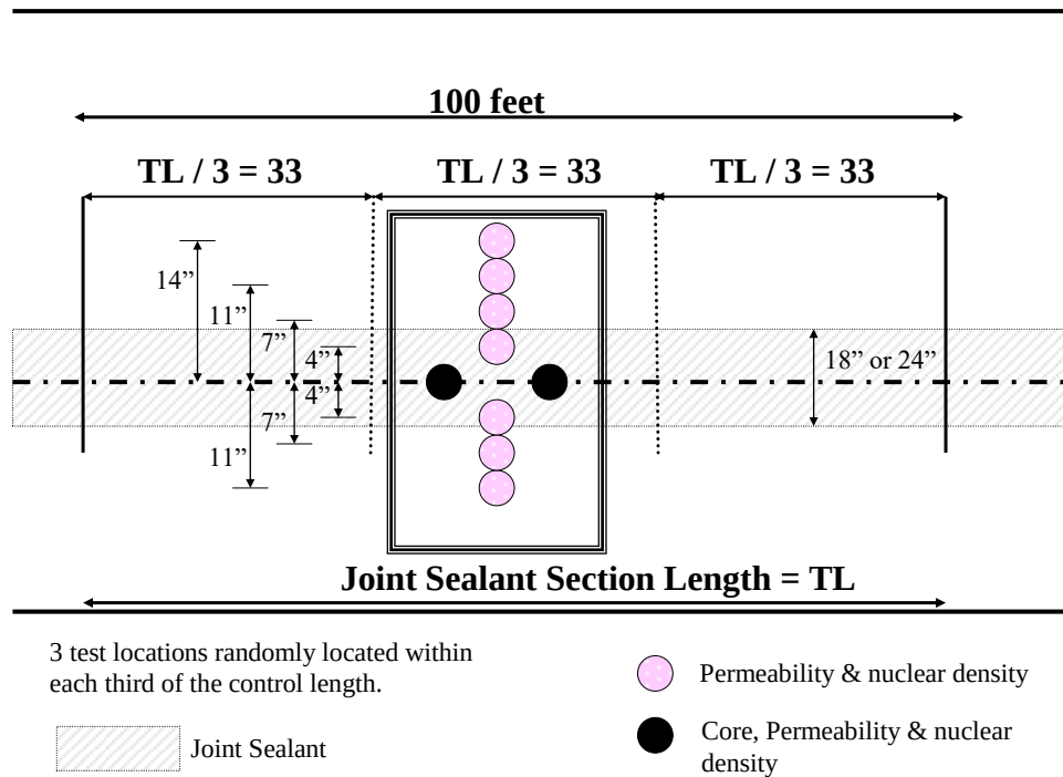
Figure 48: US 51 Joint Sealant Testing Layout
