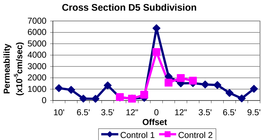
Figure 36: Subdivision Control Permeability
