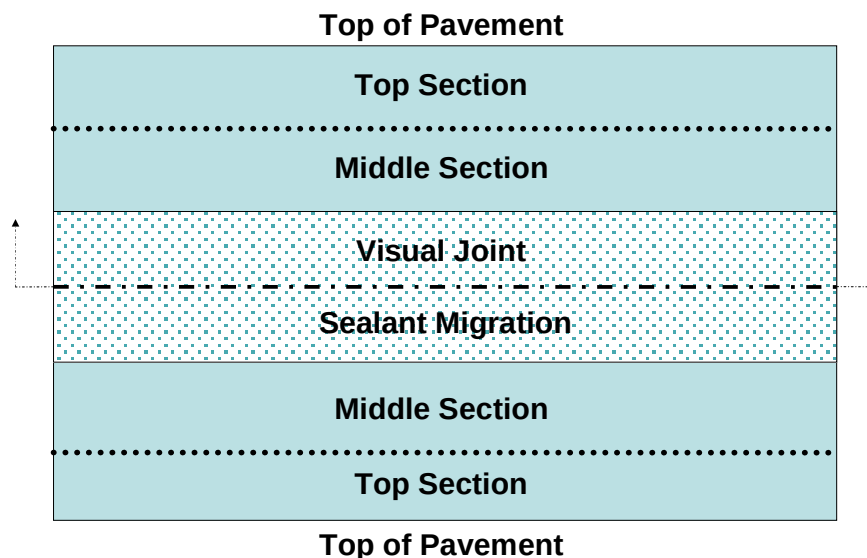
Figure 14: Core Sectioning (Core Folded in Half)
