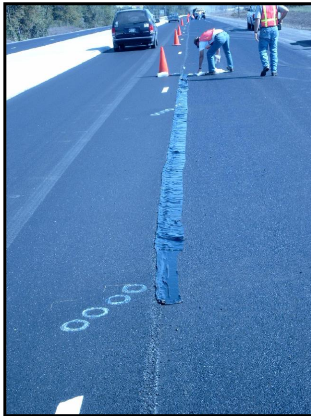
Figure 41: US 51 QuikSeam Placement
