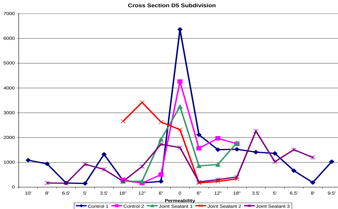
Figure 37: Subdivision Permeability Summary
