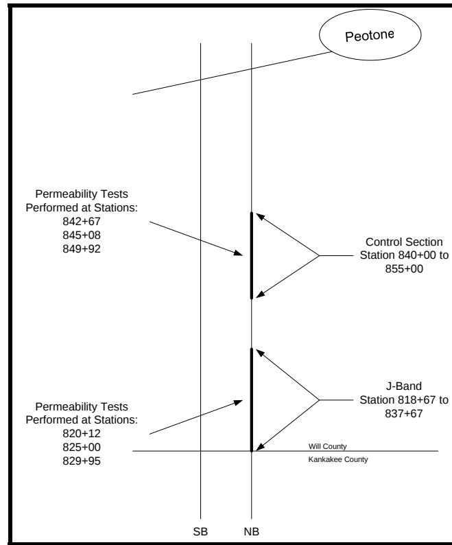
Figure 14 Interstate 57 Project Layout
