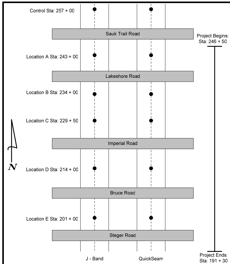
Figure 3 Illinois Route 50 Project Layout
