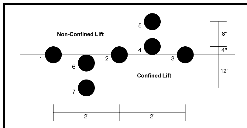
Figure 17 Permeability Testing Layout
