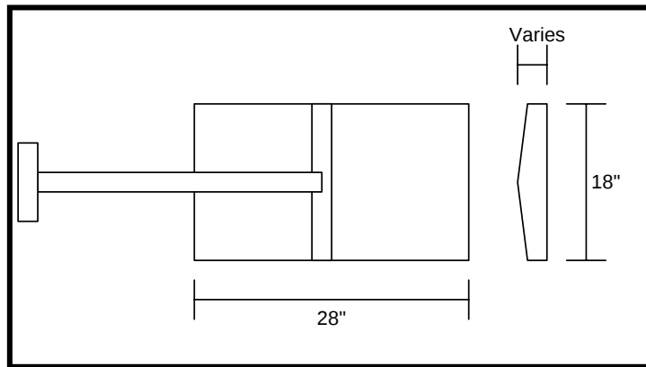
Figure 4 Schematic of J-Band® Application Tool
