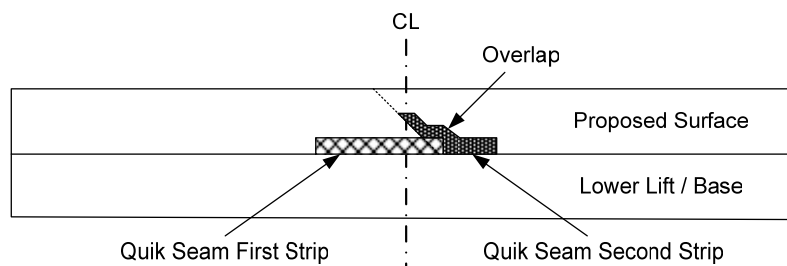
Figure 3: Quik Seam Placement
