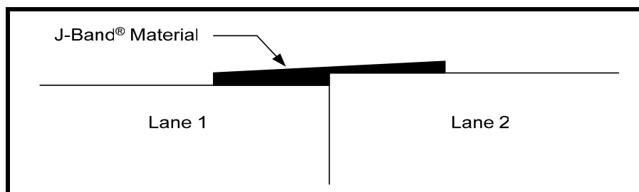
Figure 5 Lane to Lane Elevation Difference With J-Band® Placement
