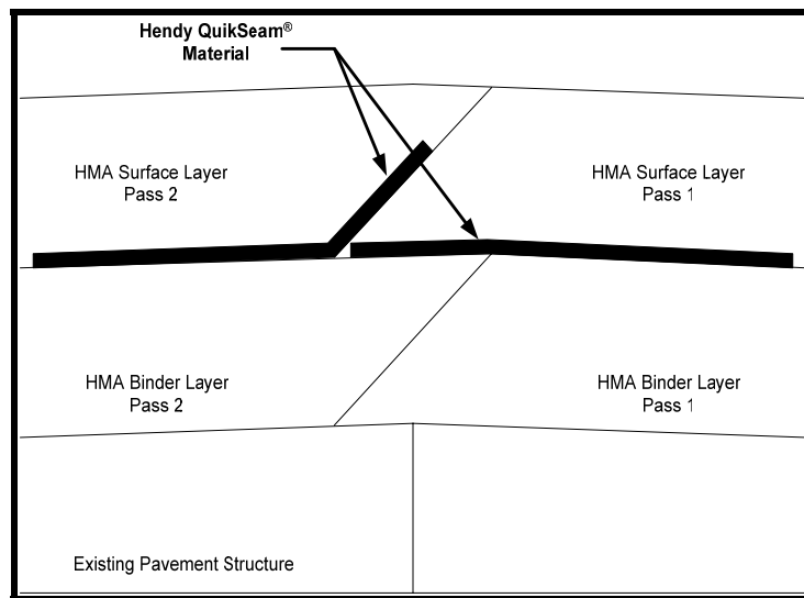
Figure 2 QuickSeam ® Material Placement
