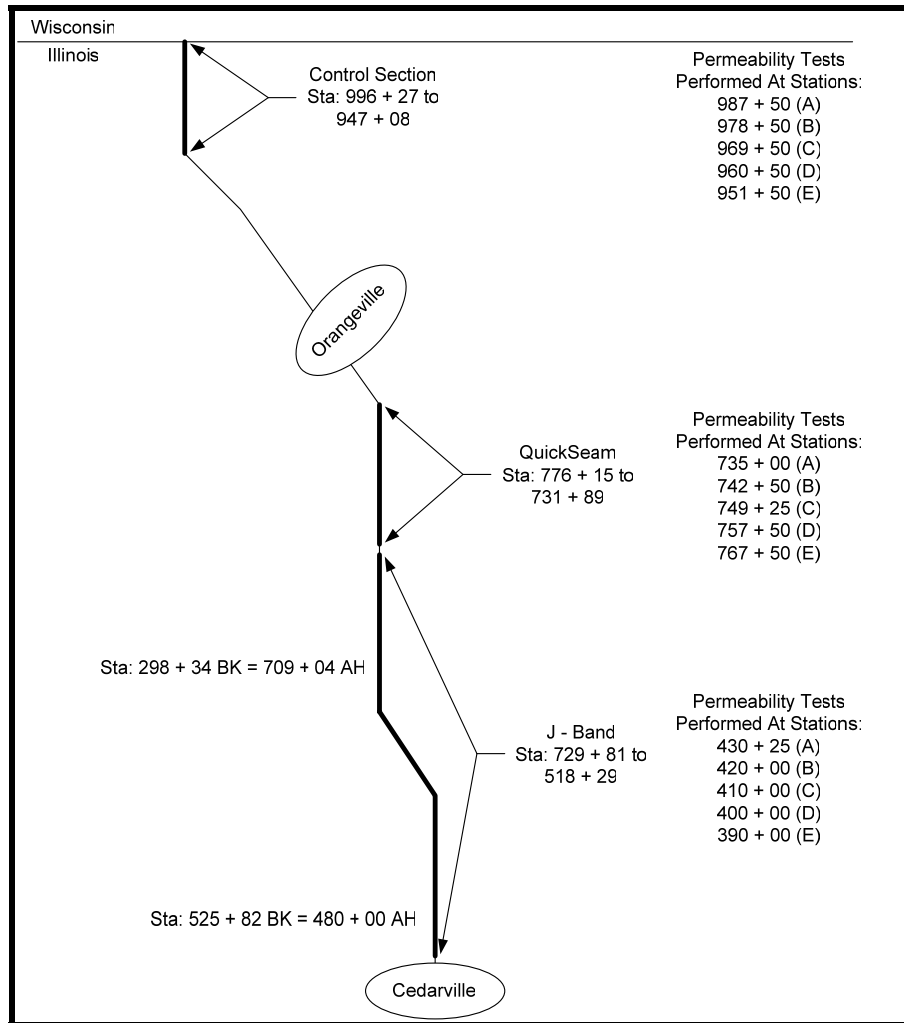
Figure 7 Illinois Route 26 Project Layout
