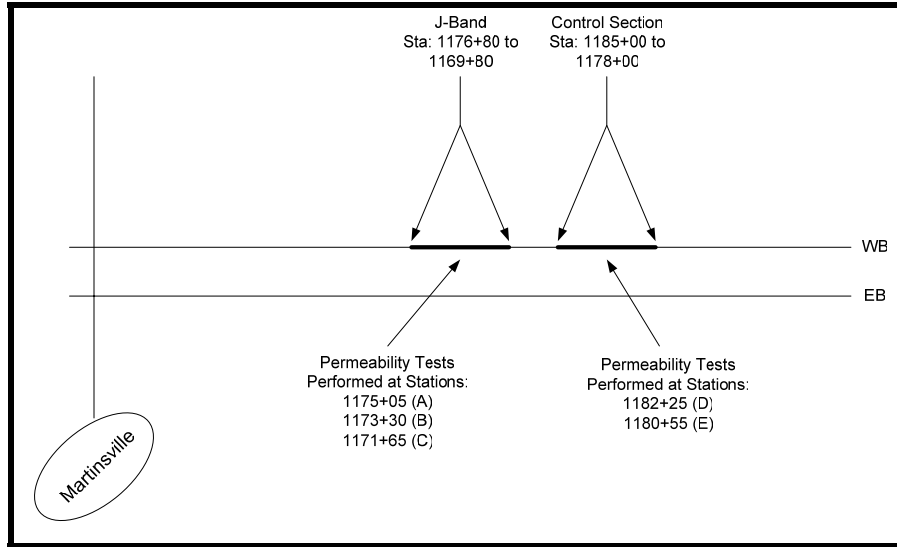
Figure 15 Interstate 70 Project Layout
