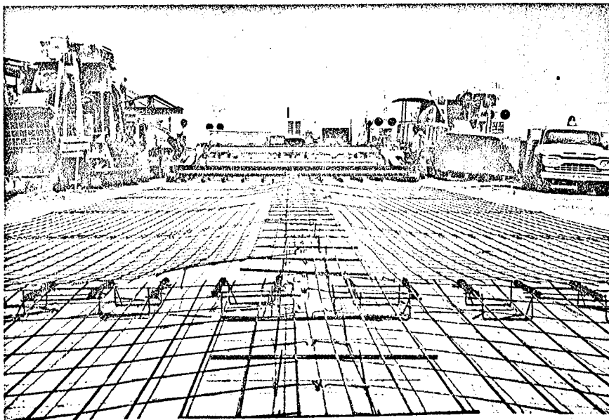
Figure 2. Wire fabric, tie bars and dowel assemblies used in unsuccessful single-lift process.
