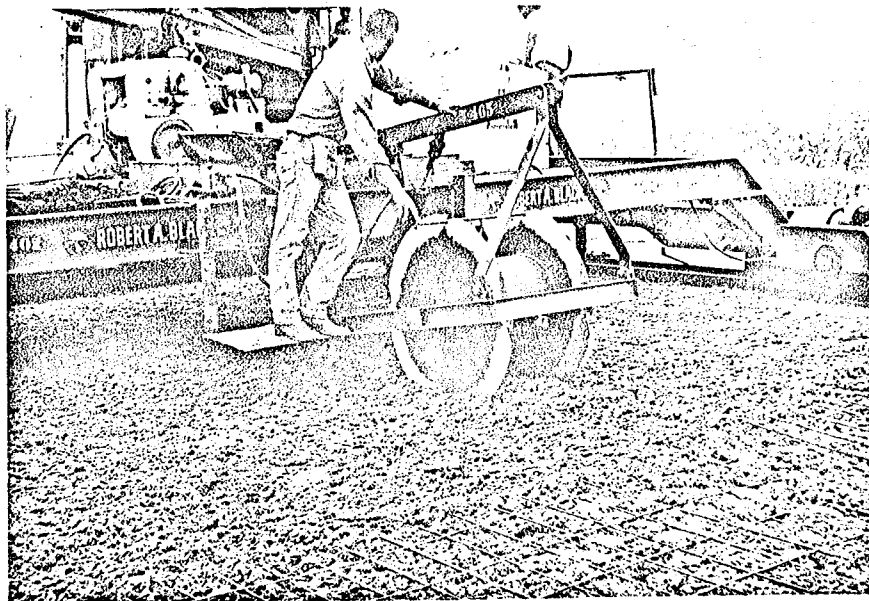
Figure 5. Tie bar placer of lead paver.
