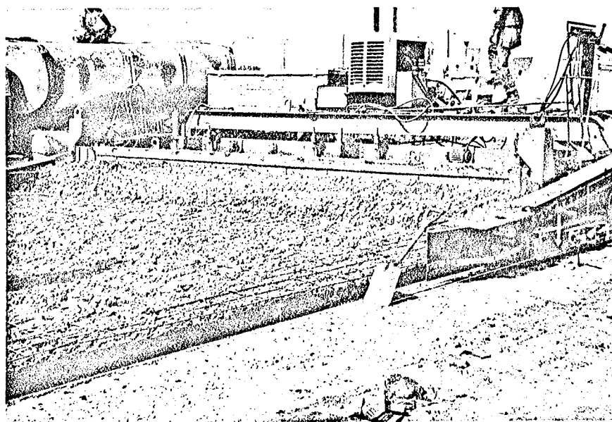
Figure 6. Second Rex slip-form paver.
