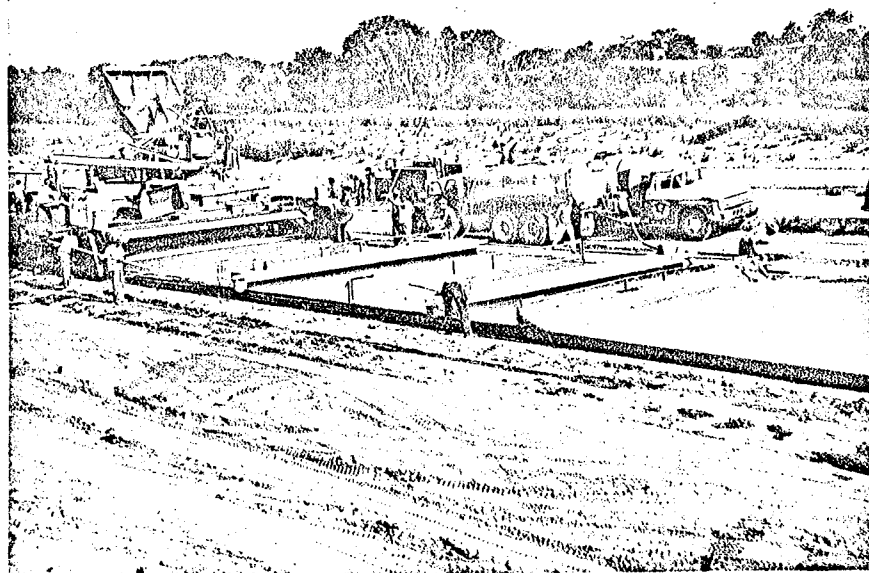
Figure 8. Finishing operations behind second paver.
