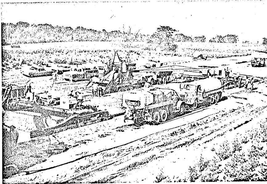
Figure 4. Rex slip-form paving train.
