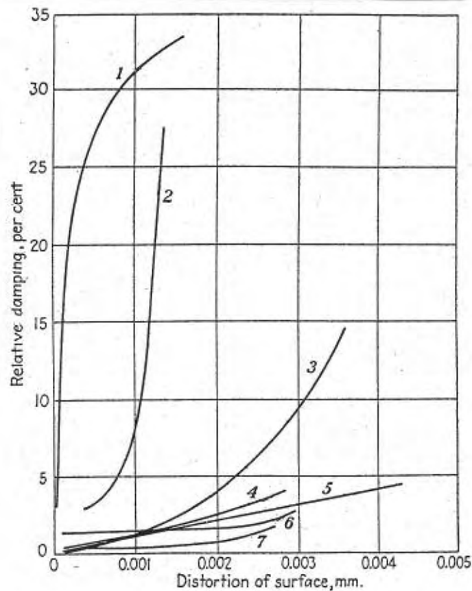
Figure 17a. Relative damping capacity of (1) gray cast iron; (2) case-hardened steel (SAE 1020); (3) silicon steel (SAE 9260); (4) nickel-manganese steel (SAE 4620); (5) nickel-chromium steel (SAE 4320; 4330; 4340); (6) chromium steel (SAE 4130; 4140); (7) red brass (CDA 836; 838). Adapted from [Ref 5].
