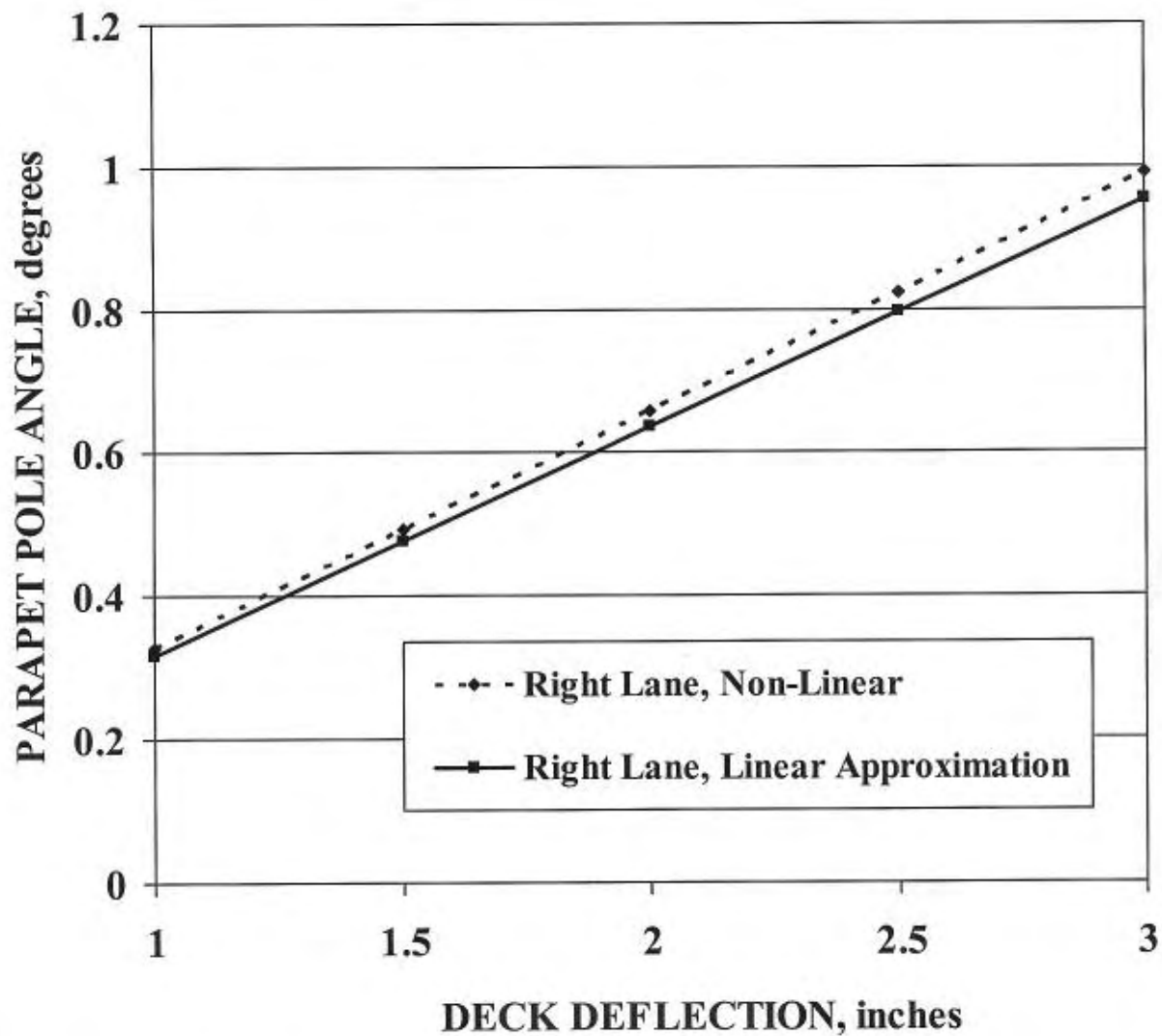
Figure 19. In this graph, the deck deflection from truck axle loads results in a deck deflection angle \theta_d , minus the parapet restraint, and is approximately equal to the pole axis deflection angle \theta_p . Conversion of deflections, using both non-linear methods and linear approximations, are plotted. Linear approximations from the tangent formula can be used for a limited range of axle loadings without generating substantial deviations from actual non-linearity.
