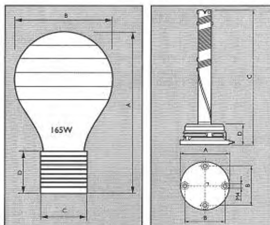
Discharge Vessel (Bulb)
