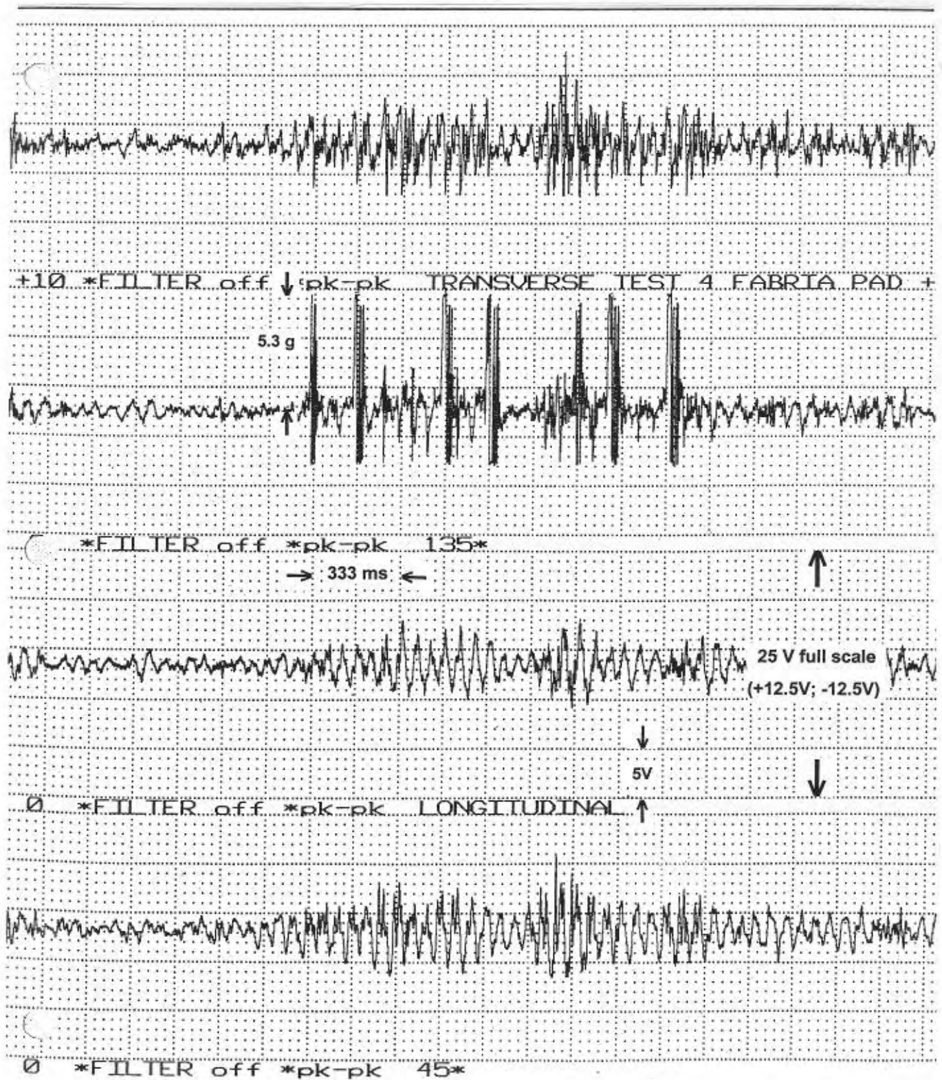
Figure 16. Oscillographic recording of the Astro-Med Dash IV of axle pulses of trucks passing by the instrumented light pole at about 55 mph. Pulses indicate the passage of two trucks, based on typical axle spacings. Calibration of the accelerometers indicated that 1V = 0.42 g. Each increment represents 33.3 milliseconds (ms), with pulse rise time at approximately 8 ms. After the initial pulse, there are additional decaying pulses from elastic rebound and vibration of the pole.
