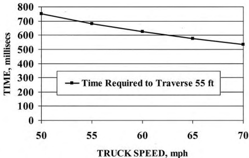
Figure 15a. The time required for the length of a typical tractor-trailer of 55 ft to pass by a lighting pole at various common truck speeds is plotted above. These times are typical cumulative durations of multiple load pulses exerted on the deck and pole by single trucks found in the oscillographic traces of accelerometer data.
