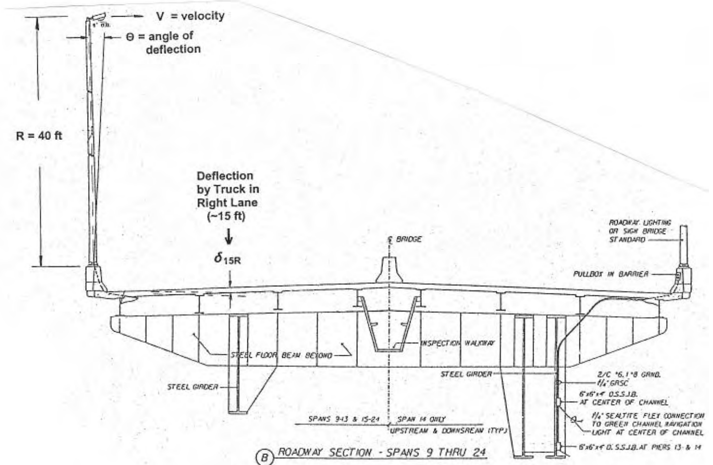
Figure 18. Typical cross section of the roadway cut between floor beams at spans 9 through 24. The deck stringers (24 WF 68) are composite with the deck between floor beams, permitting rigidity of the deck as a truck passes by. In the analysis of this report, truck axle loadings cause an approximate center loading, inducing deck deflection \delta . The deck ends are restrained by the parapet, resulting in a final net deck end angle \Theta_d . After \Theta_d is generated at the parapet, that angle results in an approximately equal pole axis angle of deflection \Theta_p .
