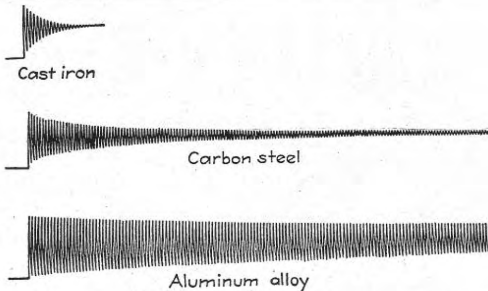
Figure 17b. Damping curves for carbon steel, aluminum alloys and gray cast iron, taken from initial deflection, subsequent oscillation, to vibration arrest, as a function of time. Damping capacity for ductile iron falls in between cast iron and carbon steel. Adapted from [Ref 6].
