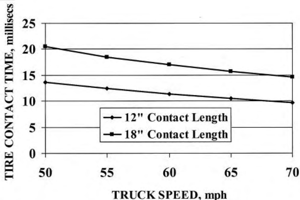
Figure 15b. The time that a truck tire is in contact with a deck length of 55 ft with with a tire contact length of 12 to 18-in. A length of 55 ft is an approximation of typical deformation zone casued by the truck. Pulses based on axle spacing, speed and time indicate that truck axles are causing localized deck deformations, triggering sharp pole vibrations.
