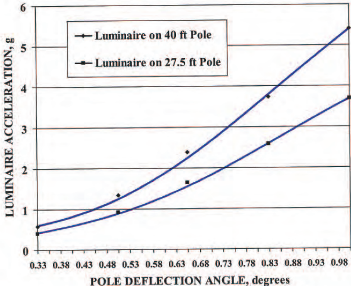
Figure 20. A plot of the accelerations experienced by luminaires mounted on the 40 ft aluminum pole, compared with a 27.5 ft pole, as a function of pole deflection angle. These accelerations are generated by load pulses of trucks passing by at 55 mph, and apply to poles mounted on the parapets. Since trucks in Illinois predominantly use the right lane, luminaires on the parapet are more vulnerable to vibration and acceleration. A shorter pole results in a lesser distance traveled by the luminaire during the pulsed deflection. Greater accelerations of luminaires would be experienced as trucks heavier than legal load pass by traveling at speeds significantly in excess of 55 mph.
